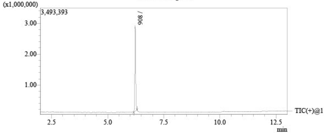
Library Search
