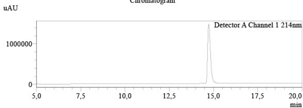
Chromatogram
